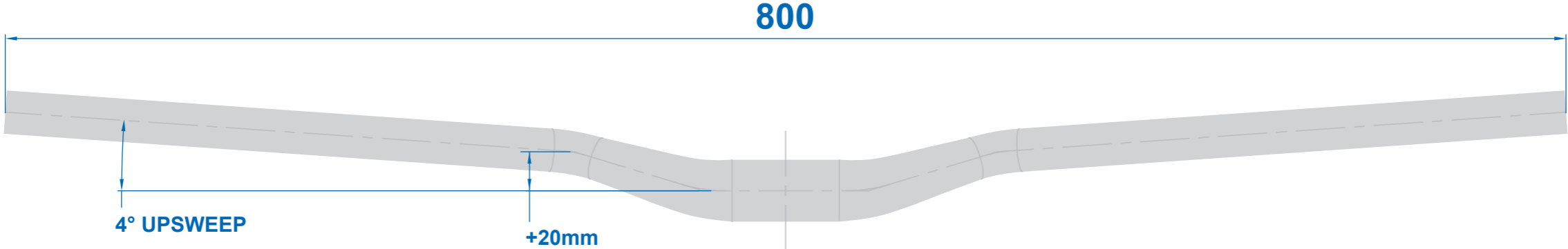
FRONT VIEW
